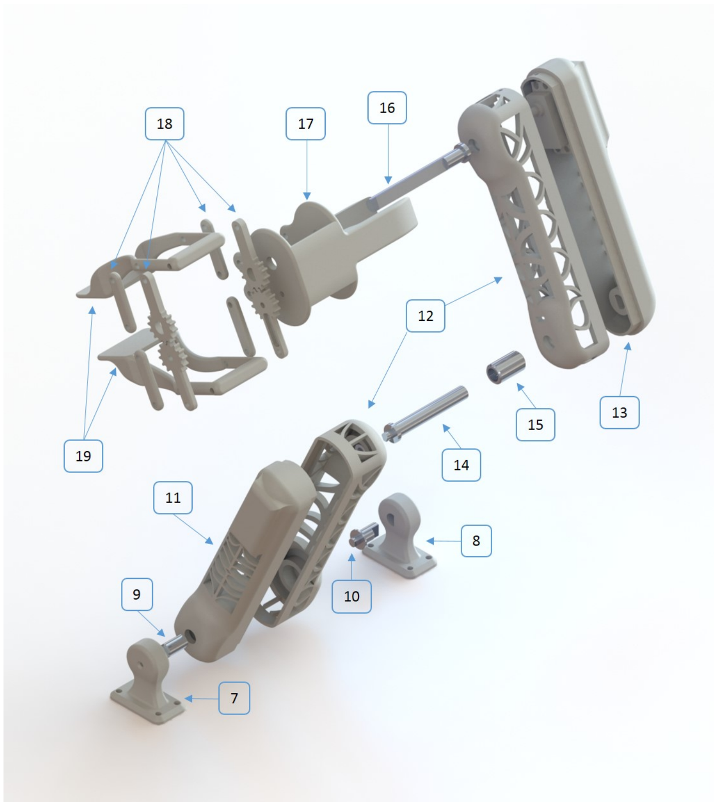
Figure 28: Exploded view of manufactured components in the Arm Assembly
