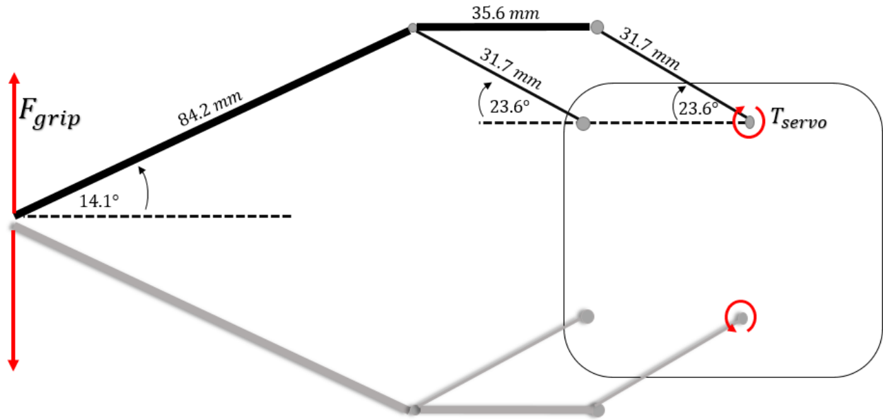
Figure 30: Rigid body force analysis for gripper mechanism
