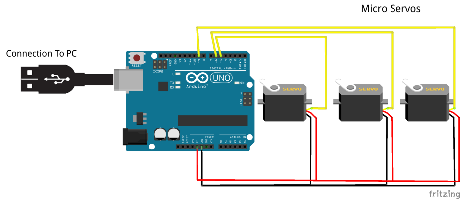
Figure 16: Schematic of the wiring for prototype 2.
