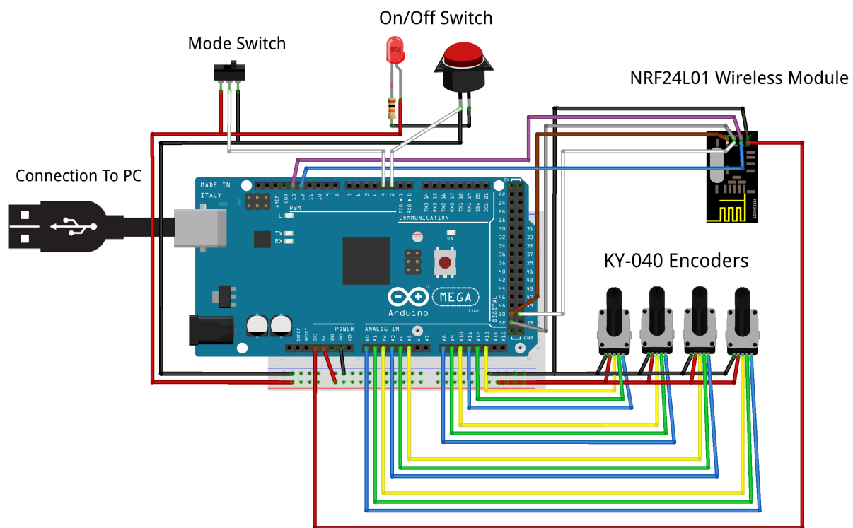
Figure 41: Wiring diagram of transmitter unit
