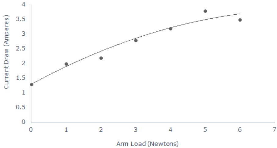
Figure 46: Graph detailing current draw increase against load increments
