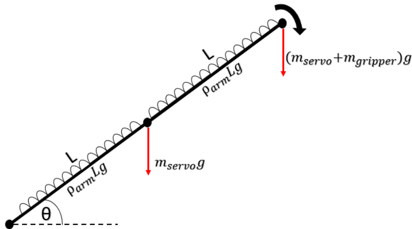
Figure 19: Rotational free body diagram for Arm
