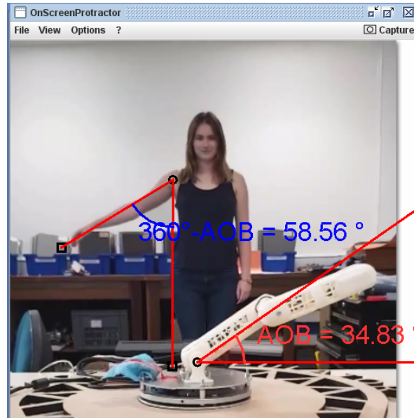
Figure 47: Image detailing use of an on screen protractor to measure the user's and robot's shoulder joint angles.
