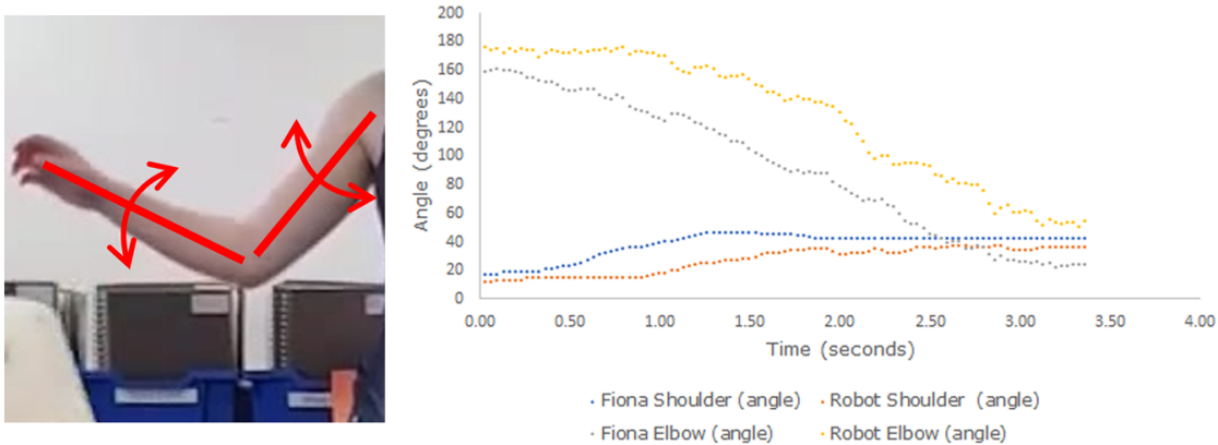
Figure 52: Scatter of multiple joint angles during dual limb motion of user and robot against time
