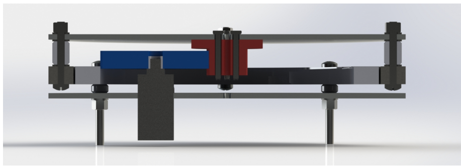
Figure 24: CAD Render of prototype 4 base plate cross-section
