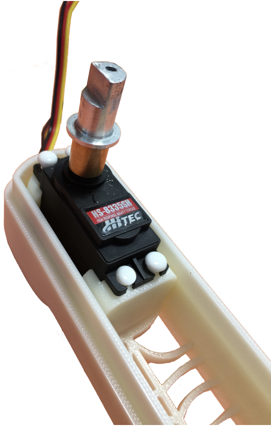
Figure 18: Servo motor in shoulder degree of freedom mounting bracket
