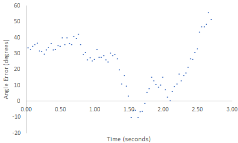
Figure 51: Scatter of elbow joint angle error
