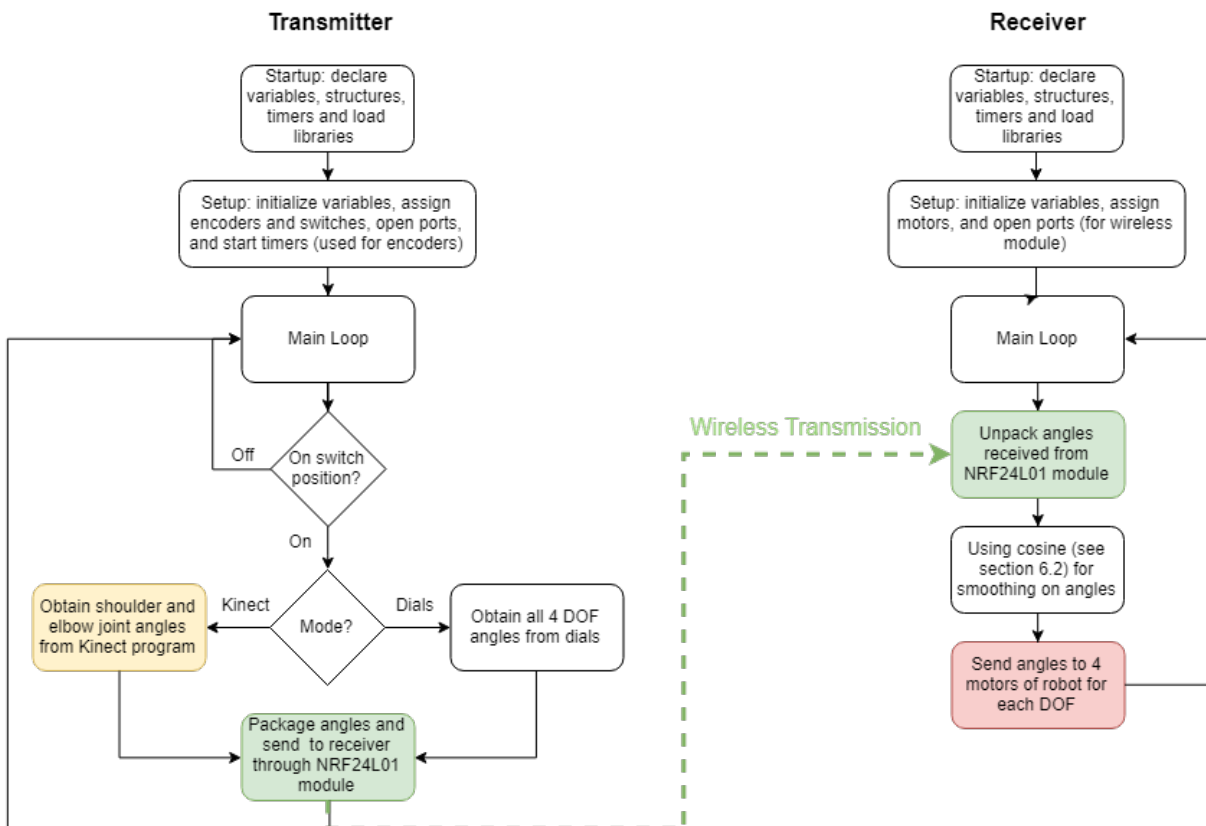
Figure 40: Flow diagram of transmitter (left) and receiver (right) programs
