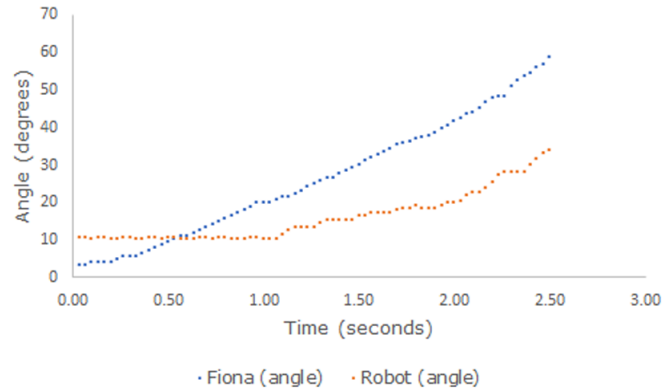
Figure 48: Scatter of joint angles during pure shoulder movement of user and robot against time
