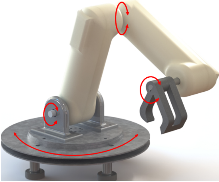
Figure 17: CAD Render of prototype 3
