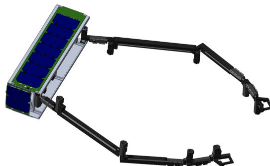
Figure 4: Solidworks model of RSat [3].
