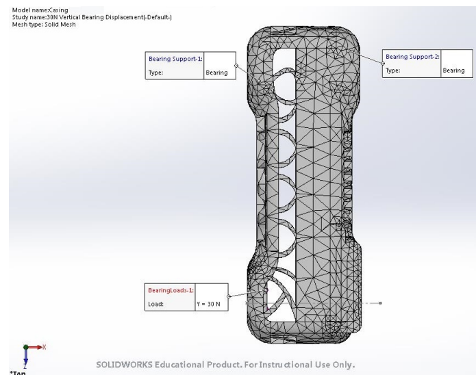
Figure 22: FE Mesh for arm section
