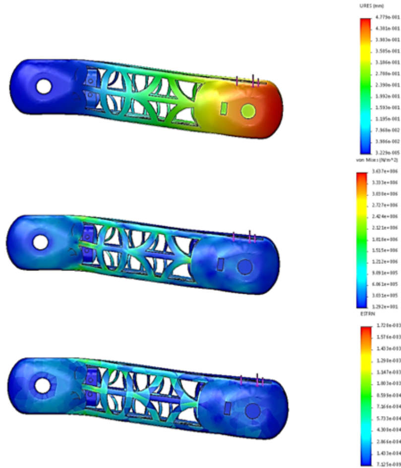
Figure 23: FE simulations for Displacement, Von-mises stress and Elastic strain for arm casing section
