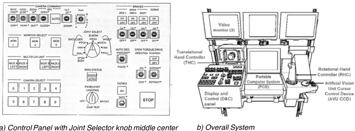
Figure 2: Schematic of Canadarm Joint Selection and Control system. [1].
