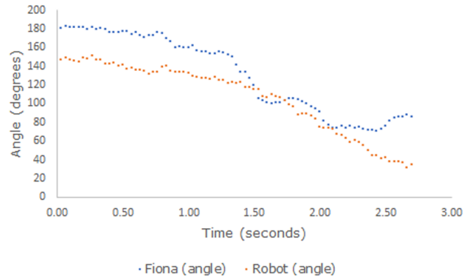
Figure 50: Scatter of joint angles during pure elbow movement of user and robot against time
