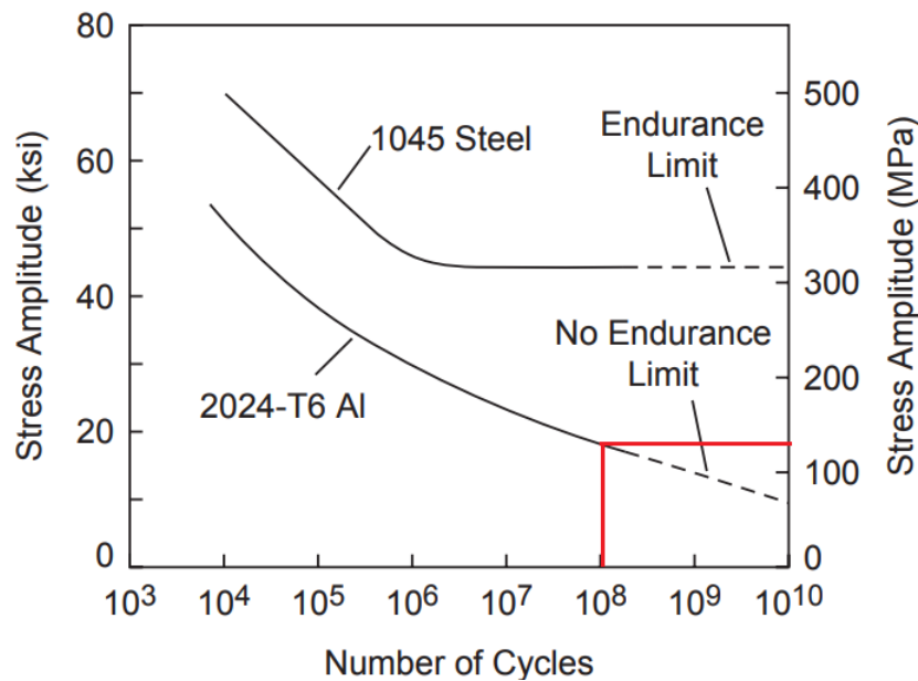
Figure 21: Fatigue curve for Aluminium [8]
