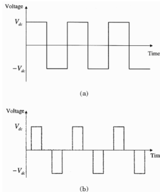
Figure 5: Example of PWM signals with different widths [4].
