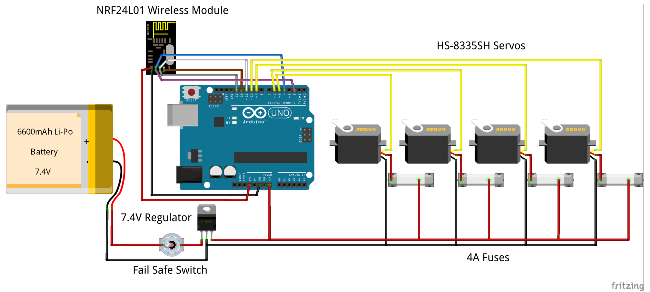
Figure 43: Wiring diagram of receiver
