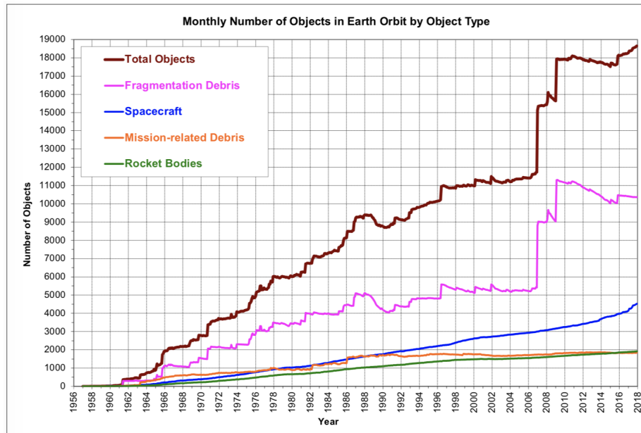
Figure 6: Graph of orbital debris per year [5].
