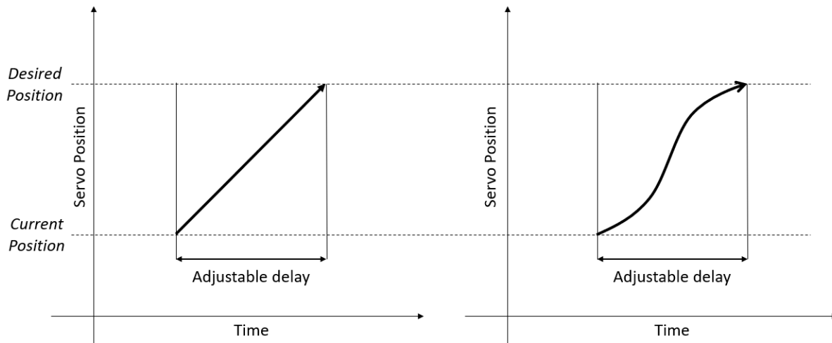
Figure 37: Linear (left) and cosine (right) adjustment of servo position over given time period
