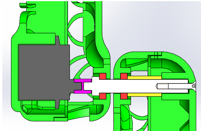
Figure 26: elbow degree of freedom cross section
