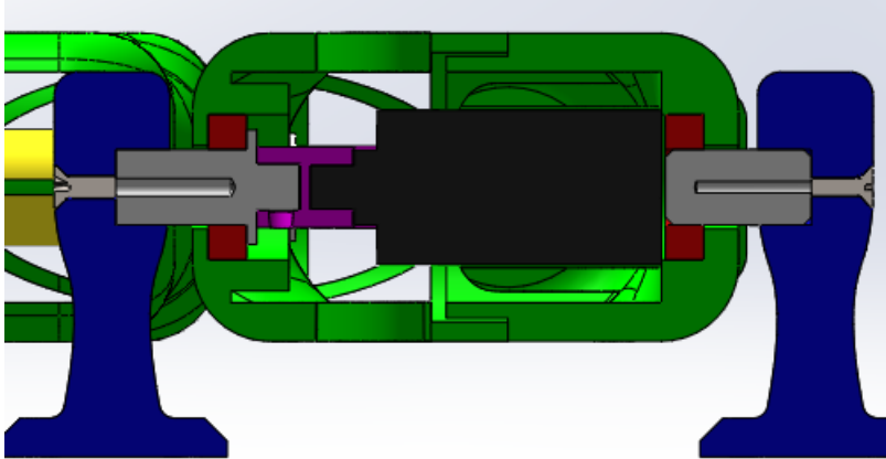
Figure 25: shoulder degree of freedom cross section
