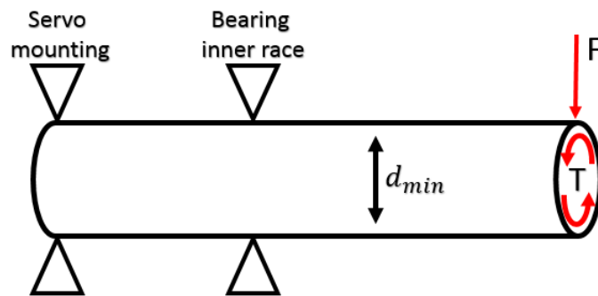
Figure 20: Simplified constraint and loading diagram of shoulder degree of freedom shaft
