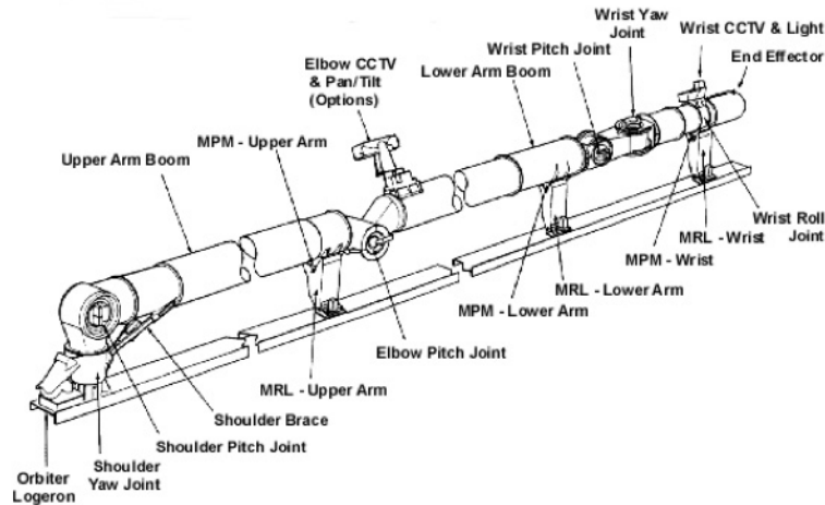
Figure 3: Schematic of Canadarm [2].
